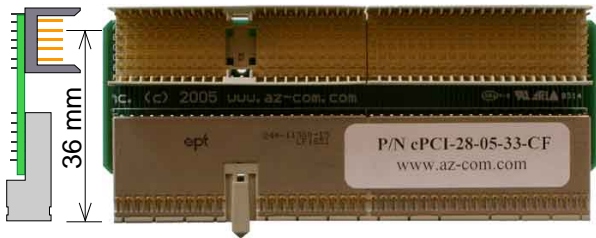
P/N cPCI-28-05-33-CF Right Angle Male top
