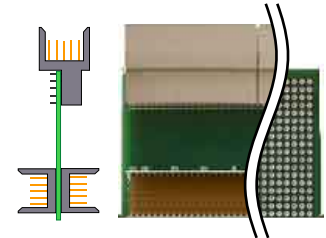
P/N cPCI-M48R-01-CFR Includes Front and Rear I/O connectors below top connector.
